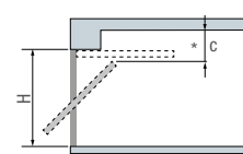
BM – Fully retracting, protruding overhead garage door.
