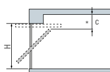
BC – Partially retracting, protruding overhead garage door. (con 001V201)
