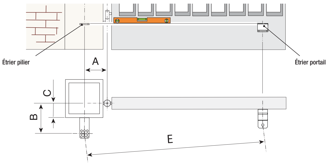
Dimensions application (mm)
